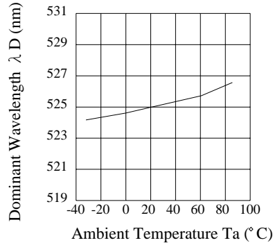
Ambient Temperature vs. Dominant Wavelength
