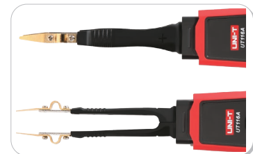
The pen can be rotated by 180° for easy reading and operation
