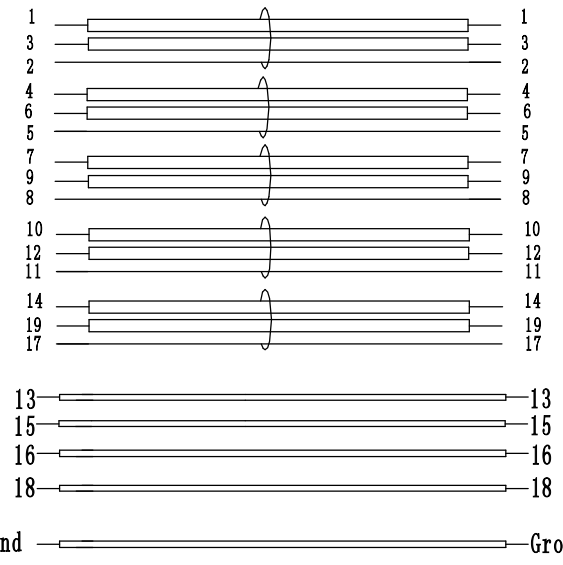
Wiring Diagram
