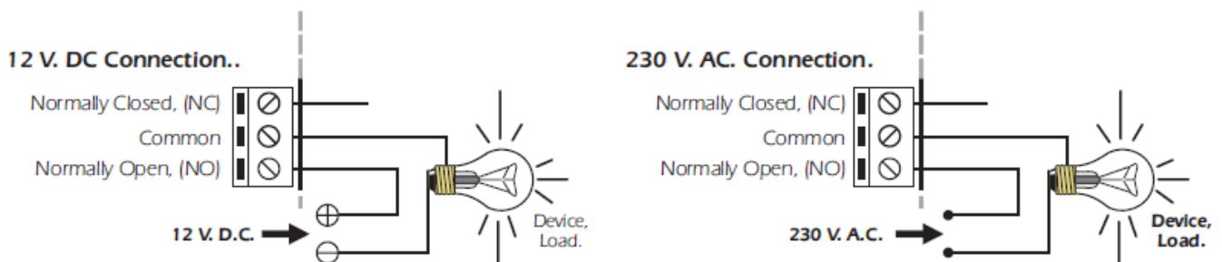
Pic. 1. 12 V. DC and 230 V. AC. connections of the module's output.
